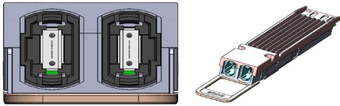
Figure 3. Optical lane assignments
