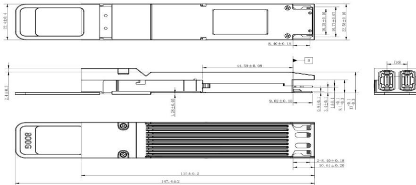
Figure 4. Mechanical Dimensions
